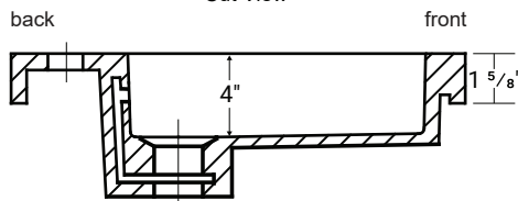
Cut View
